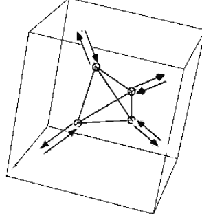
Figure 3: The local ground state of the generalized NJL-model eqs.(18) and (15). The total of 8 internal spin vectors accounts for 3 \times 8 d.o.f. corresponding to 24 spin vibrations which can be classified according to the multiplet structure of the Shubnikov group, eq.(17). The vectors \vec{S}_i^0 are assumed to point outwards and \vec{T}_i^0 = -\vec{S}_i^0 inwards. According to eq. (12) this corresponds to \langle \psi^\dagger \gamma_5 \vec{\tau} \psi \rangle_i \neq 0 . The alternative vacuum configuration (16) where \langle \psi^\dagger \vec{\tau} \psi \rangle_i \neq 0 and the \vec{T}_i^0 are parallel to the \vec{S}_i^0 instead of anti-parallel is not drawn.
