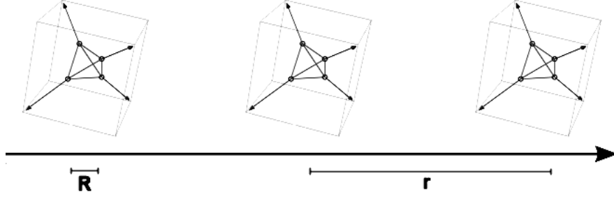
Figure 2: The global ground state of the model after SSB consists of an aligned system of chiral tetrahedrons over Minkowski space (the latter represented by the long arrow). R is the magnitude of one tetrahedron and r the distance between two of them. Note that contrary to what is drawn here, the tetrahedra extend into internal space alone, not into Minkowski space. Before the SSB the chiral tetrahedrons are oriented randomly (not shown) and there is a corresponding local SO(3) symmetry, because each rigid tetrahedron can be rotated freely and independently from the others.
